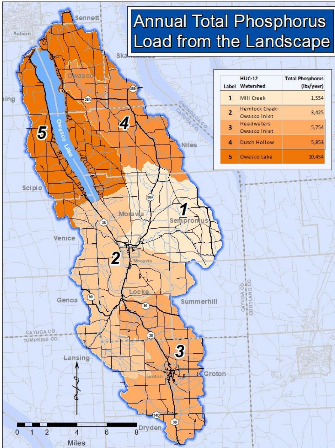
Figure 10: Baseline SWAT Model Projection: Estimated Annual Total Phosphorus Load by Subwatershed
