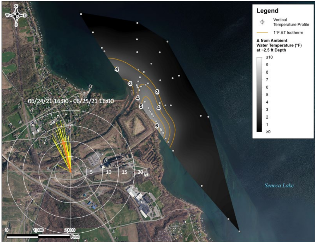
Figure 4-9 Interpolated surface \Delta T isotherms from tri-axial survey conducted on June 25, 2021. Interpolated area with greater than 3°F rise in surface temperature is 38.4 acres. Wind rose shows wind velocity (mph) and direction over a 24-hour period ending with the survey.
