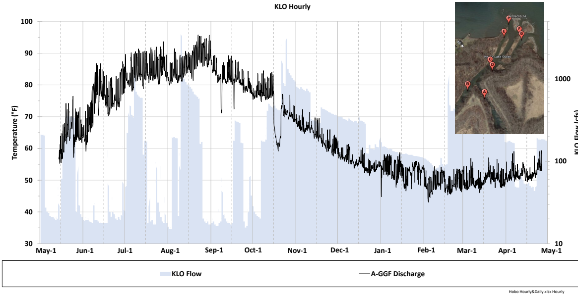
Figure 4-5 Observed hourly GGF discharge temperature at Station A.
