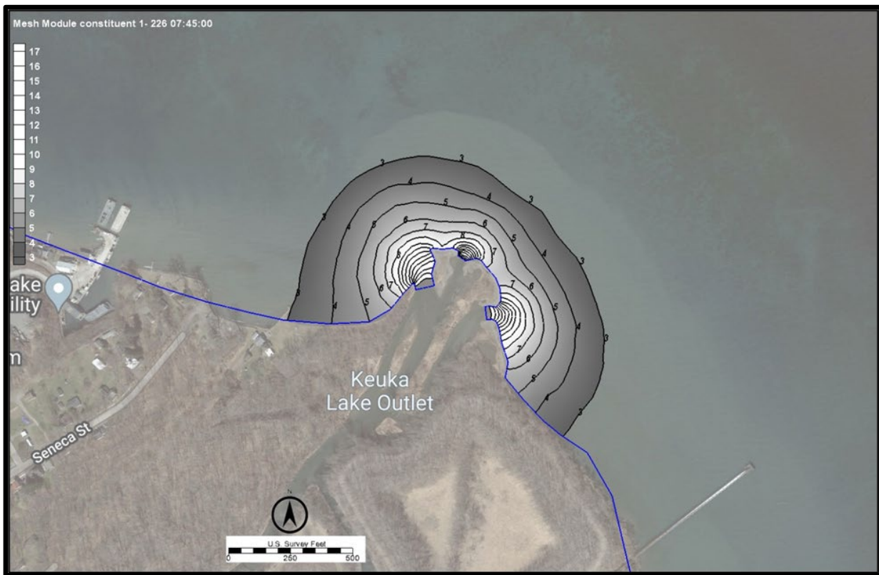
Figure 6.10: \Delta T Contours for Scenario Simulation 8 at 8/14/21 07:45. (Background Air Temp also increase by 6 Degrees F). The enclosed area where \Delta T is \geq 3^\circ\text{F} is 15.5 Acres
