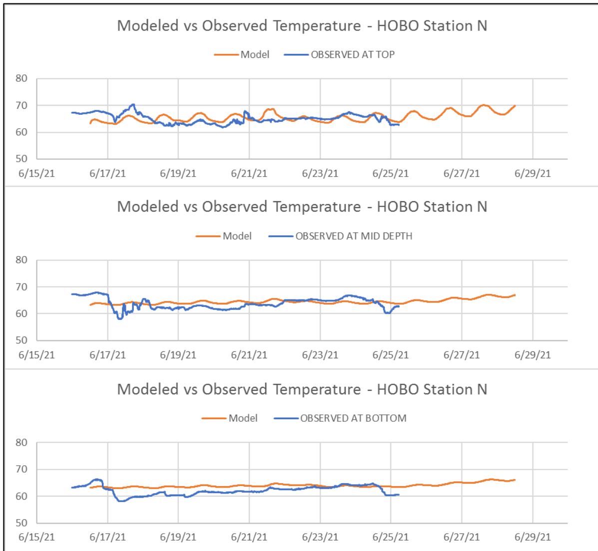
Figure 4.9: Model calibration results at HOB0 Station N
