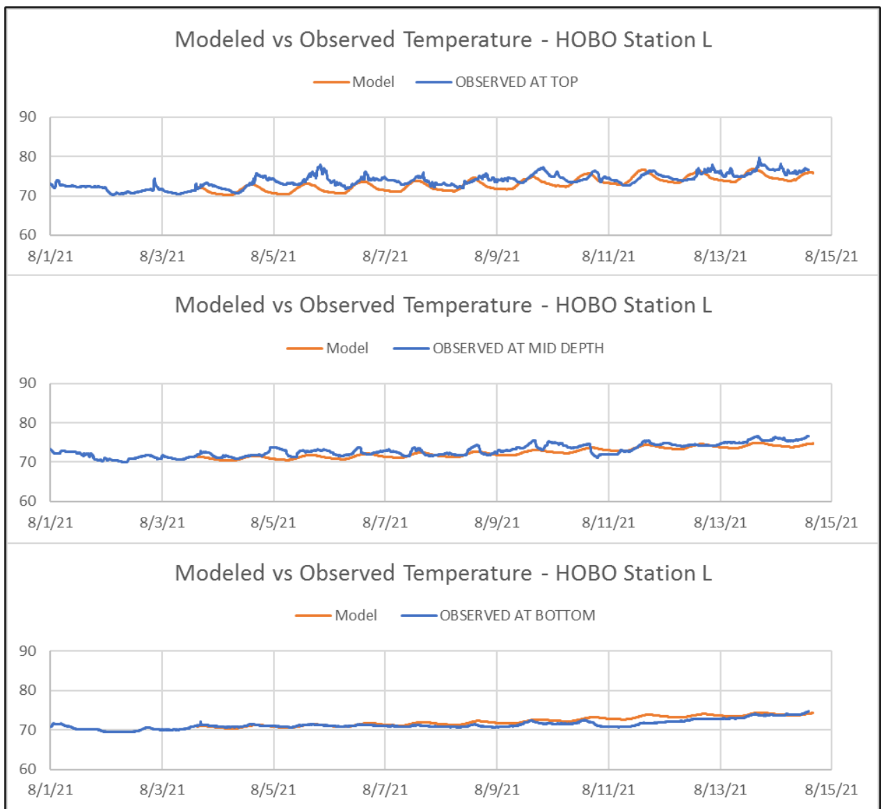
Figure 5.6: Model verification results at HOB0 Station L
