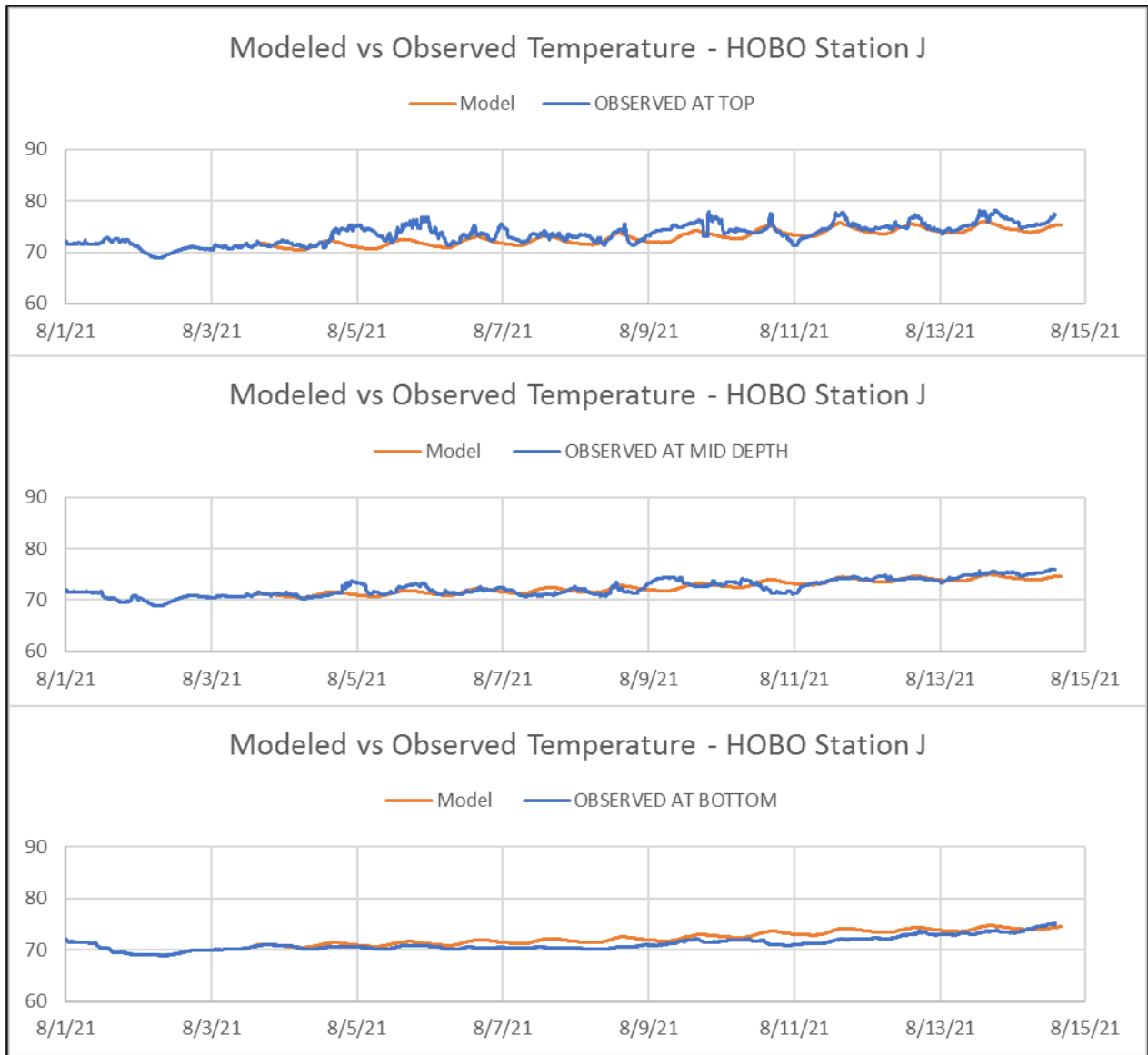
Figure 5.4: Model verification results at HOB0 Station J
