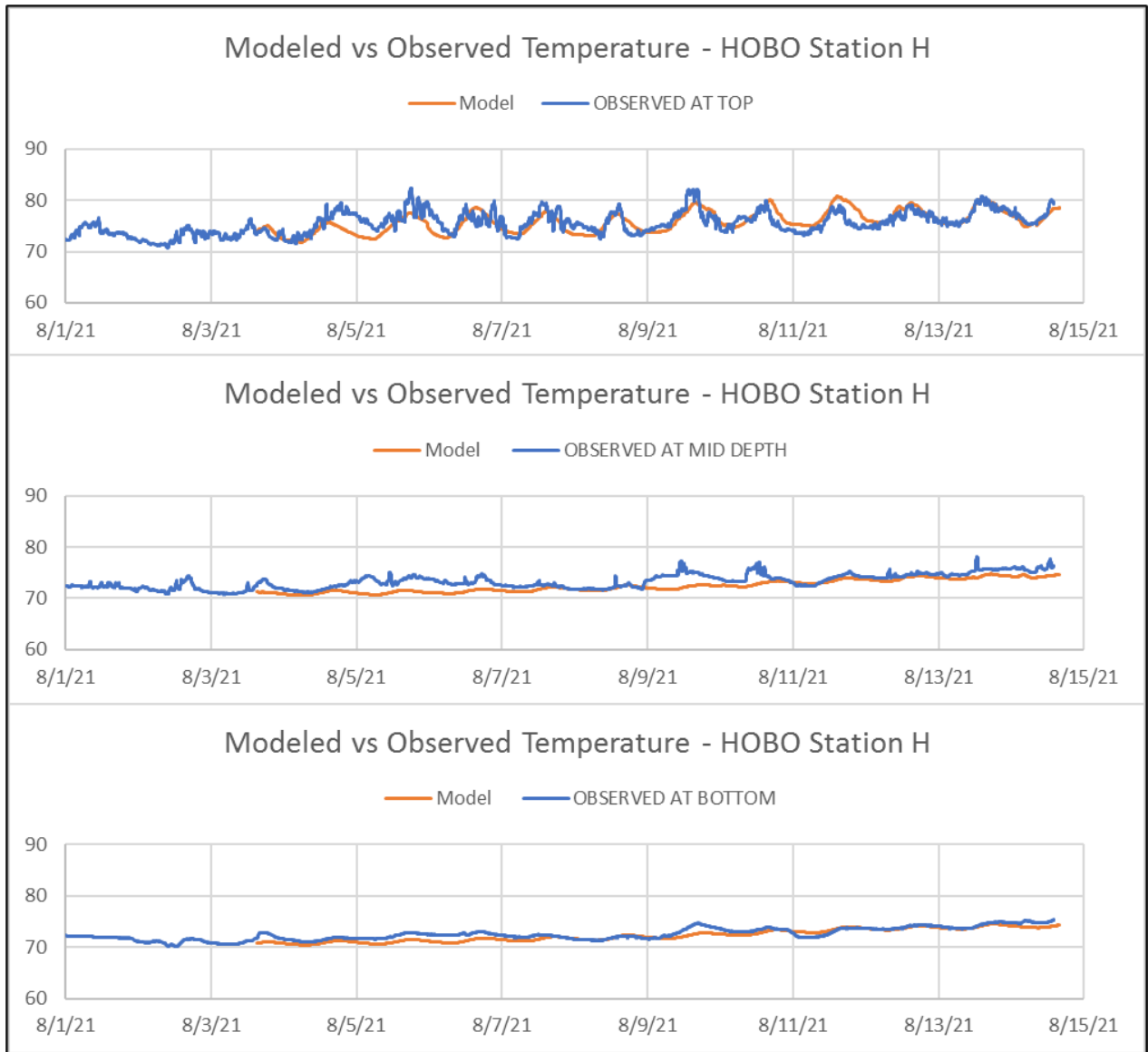
Figure 5.1: Model verification results at HOB0 Station H
