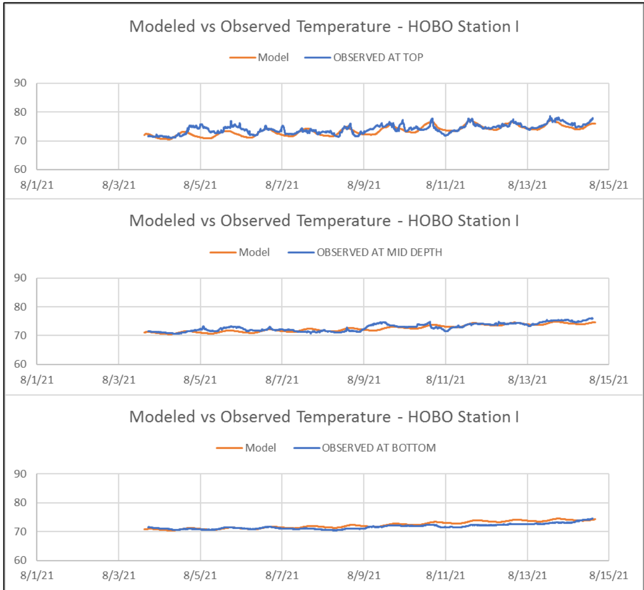
Figure 5.3: Model verification results at HOB0 Station I
