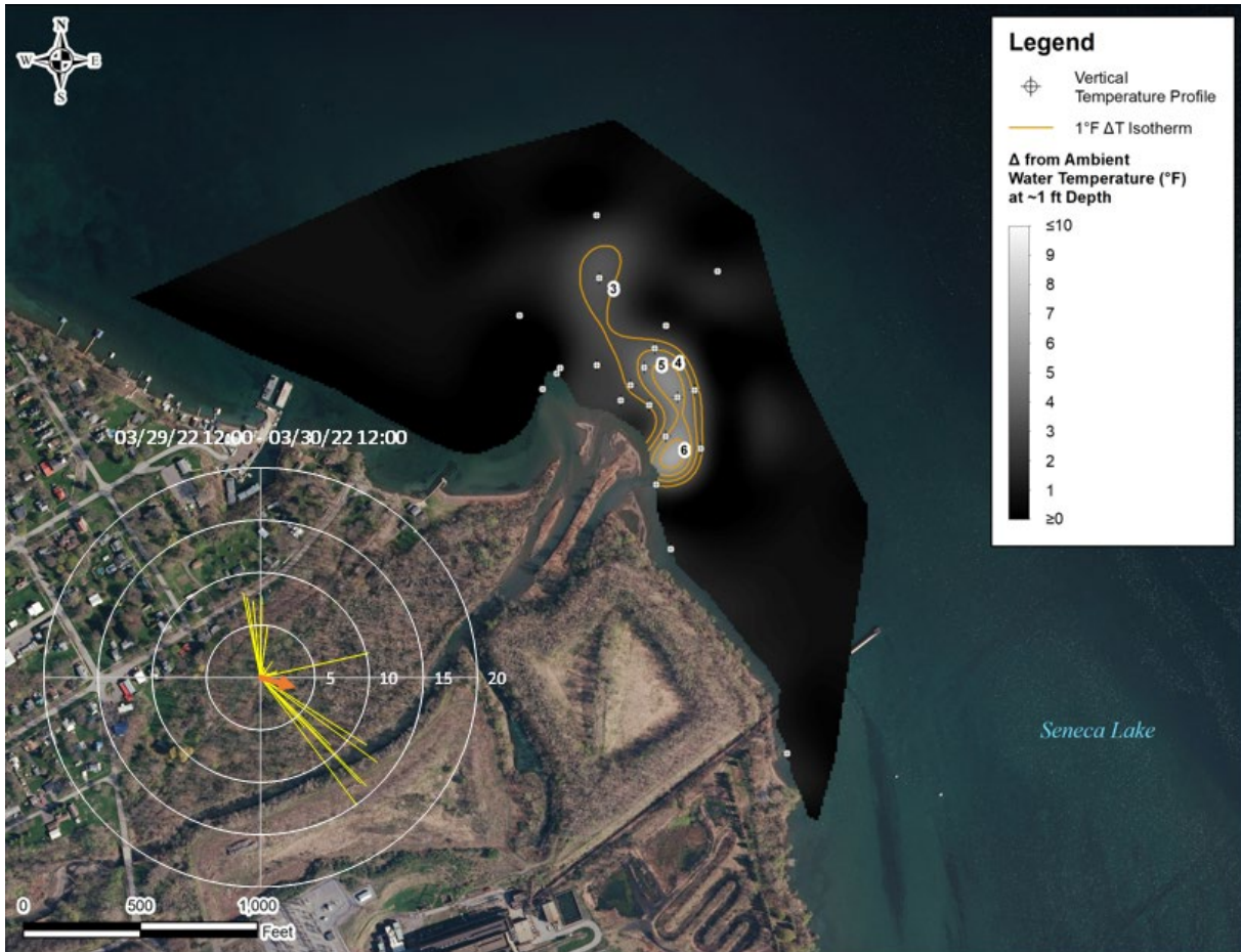
Figure 4-16 Interpolated surface isotherms from tri-axial survey conducted on March 30, 2022. Interpolated area with greater than 3°F rise in surface temperature is 4.3 acres. Wind rose shows wind velocity (mph) and direction over a 24-hour period ending with the survey.
