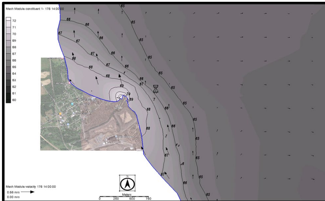
Figure 4.13: Model calibration simulation of surface water temperatures on 6/26/21 at 13:00 hours.
