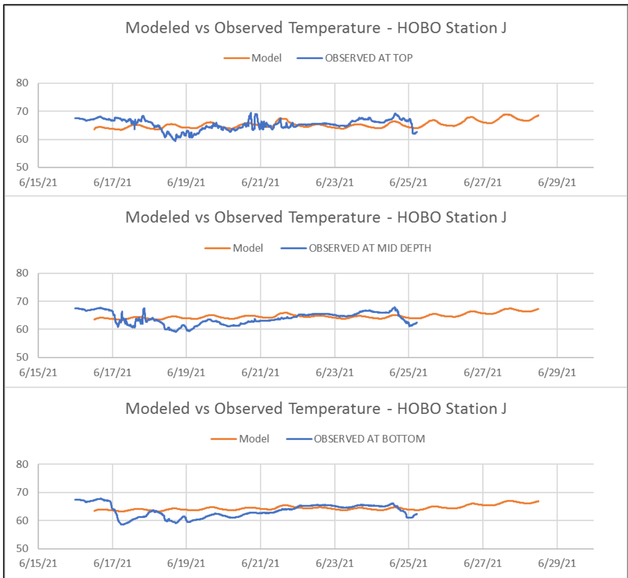
Figure 4.5: Model calibration results at HOB0 Station J
