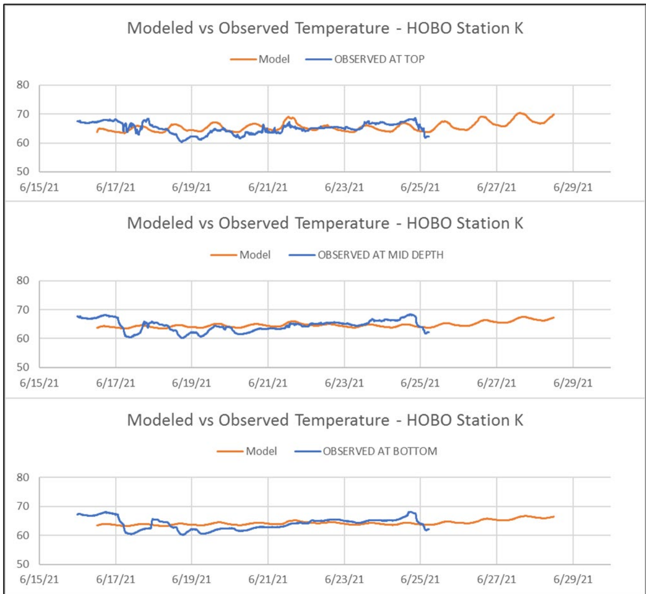
Figure 4.6: Model calibration results at HOB0 Station K
