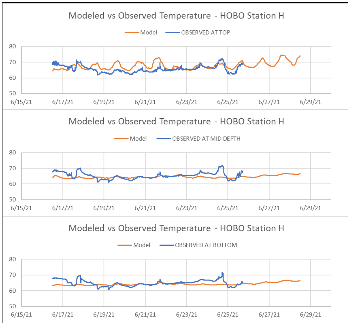
Figure 4.2: Model calibration results at HOB0 Station H
